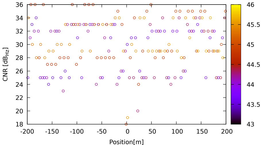
CNR vs position for C33 (B1) on HuaweiP40 - DOY 263 jam. 2
