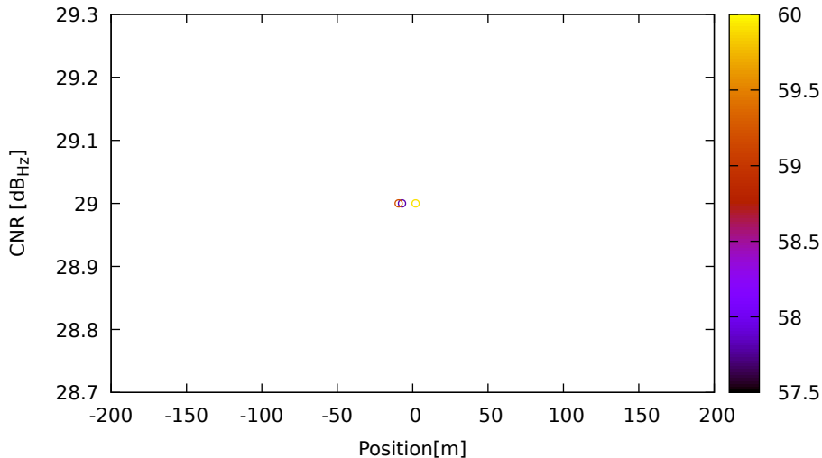
CNR vs position for E04 (E5a) on HuaweiP40 - DOY 263 jam. 2
