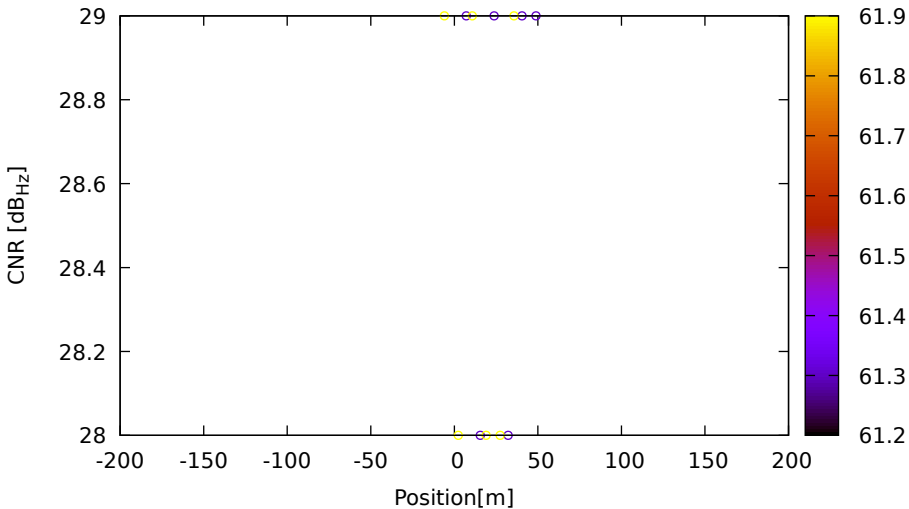
CNR vs position for E04 (E5a) on HuaweiP40 - DOY 263 jam. 3
