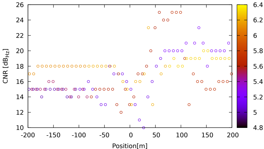
CNR vs position for E09 (E1) on HuaweiP40 - DOY 263 jam. 1
