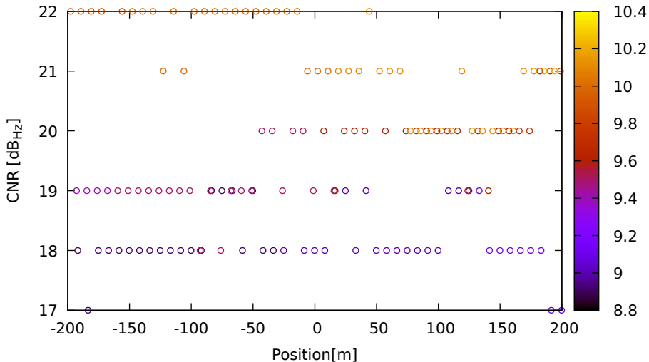
CNR vs position for E09 (E1) on HuaweiP40 - DOY 263 jam. 3
