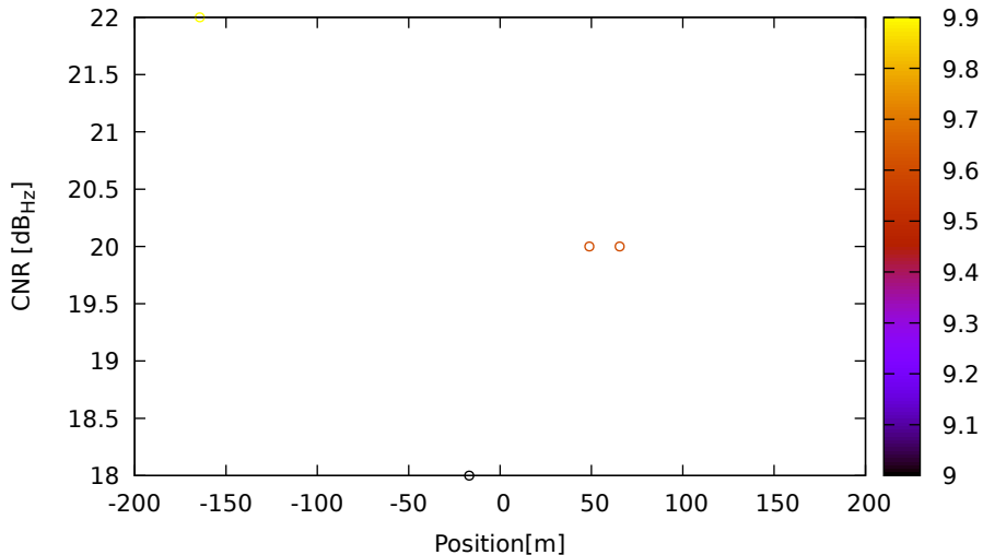
CNR vs position for E09 (E5a) on HuaweiP40 - DOY 263 jam. 3
