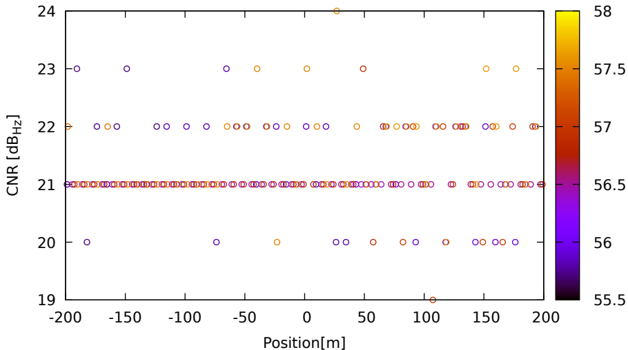
CNR vs position for E11 (E1) on HuaweiP40 - DOY 263 jam. 2
