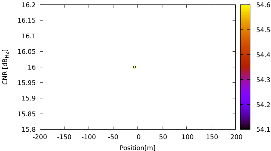
CNR vs position for E11 (E5a) on HuaweiP40 - DOY 263 jam. 1
