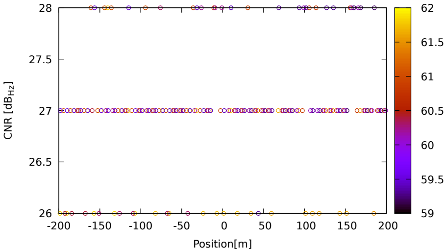
CNR vs position for E12 (E1) on HuaweiP40 - DOY 263 jam. 2
