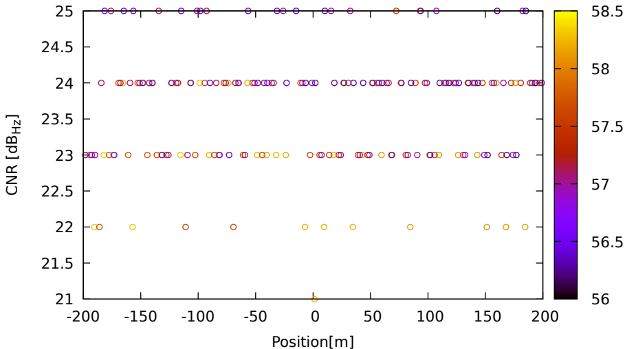
CNR vs position for E19 (E1) on HuaweiP40 - DOY 263 jam. 2
