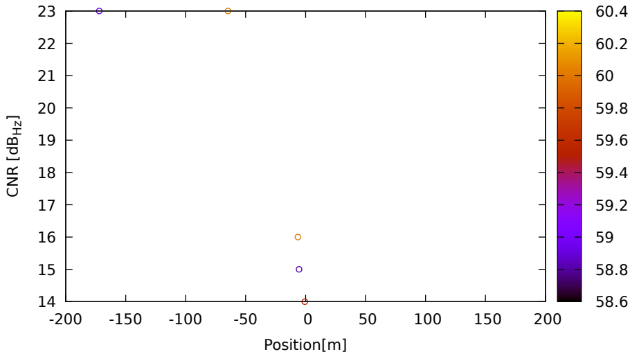
CNR vs position for E19 (E5a) on HuaweiP40 - DOY 263 jam. 1
