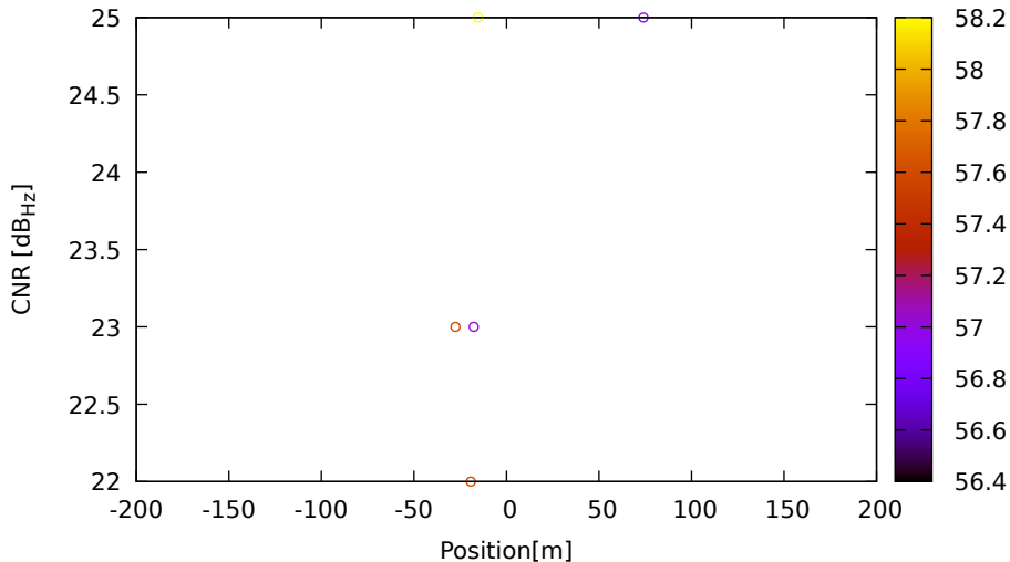
CNR vs position for E19 (E5a) on HuaweiP40 - DOY 263 jam. 2
