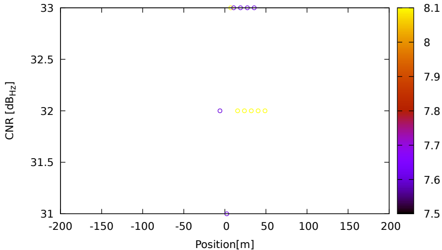
CNR vs position for E33 (E5a) on HuaweiP40 - DOY 263 jam. 3
