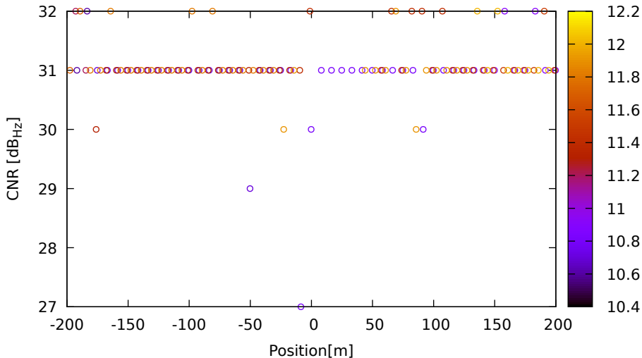
CNR vs position for E36 (E1) on HuaweiP40 - DOY 263 jam. 3
