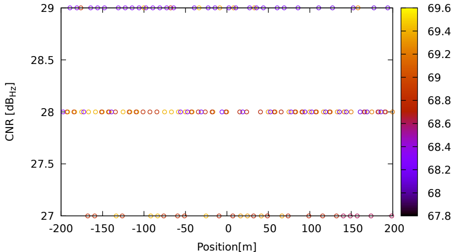
CNR vs position for G03 (L5) on HuaweiP40 - DOY 263 jam. 3
