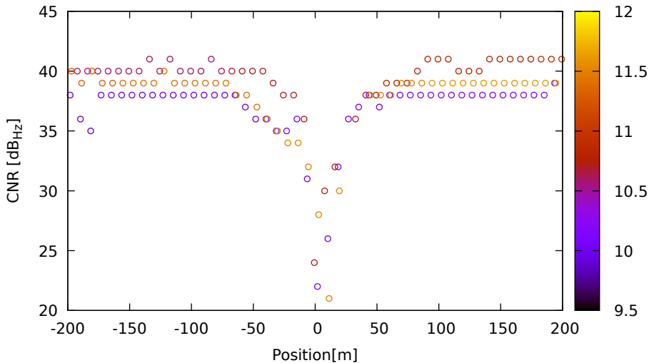
CNR vs position for G06 (L1) on HuaweiP40 - DOY 263 jam. 1
