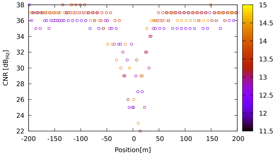
CNR vs position for G06 (L1) on HuaweiP40 - DOY 263 jam. 2
