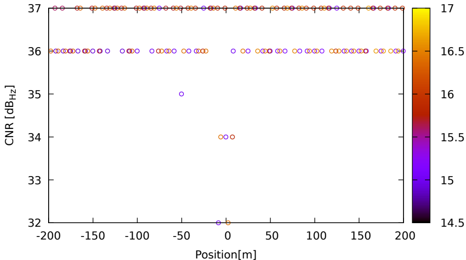
CNR vs position for G06 (L5) on HuaweiP40 - DOY 263 jam. 3
