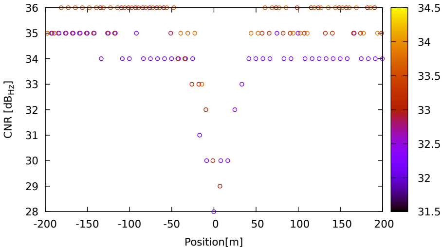
CNR vs position for G09 (L1) on HuaweiP40 - DOY 263 jam. 3
