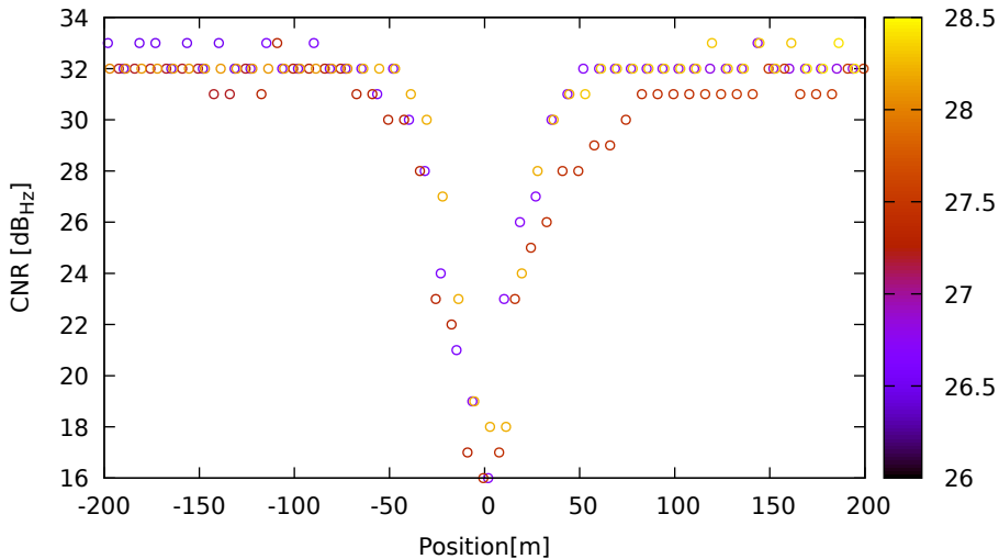
CNR vs position for G09 (L5) on HuaweiP40 - DOY 263 jam. 1
