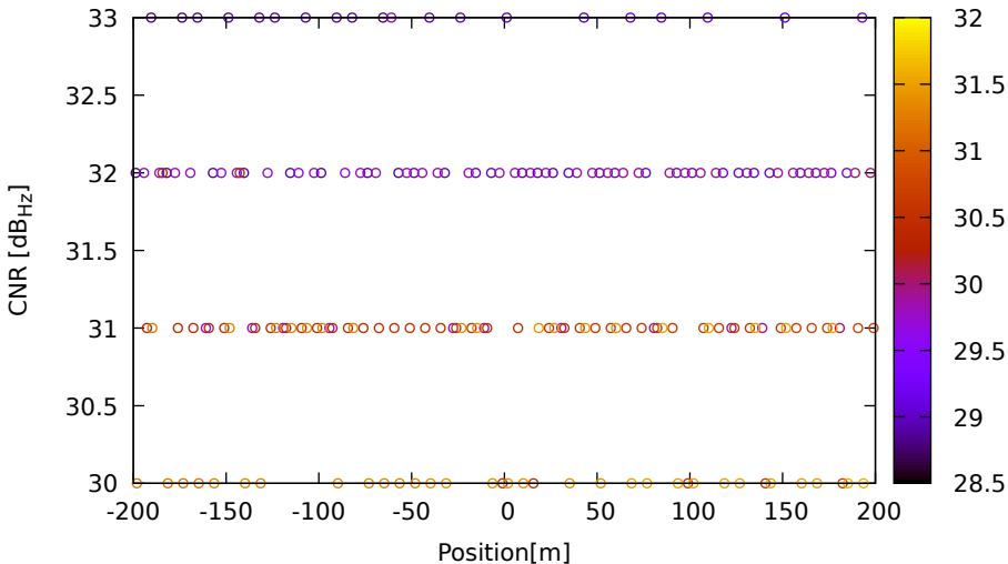
CNR vs position for G09 (L5) on HuaweiP40 - DOY 263 jam. 2
