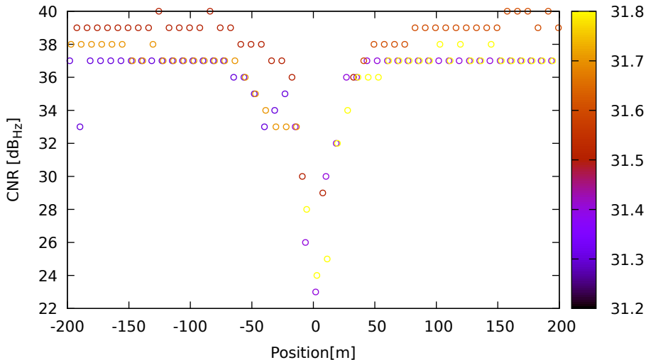
CNR vs position for G19 (L1) on HuaweiP40 - DOY 263 jam. 1
