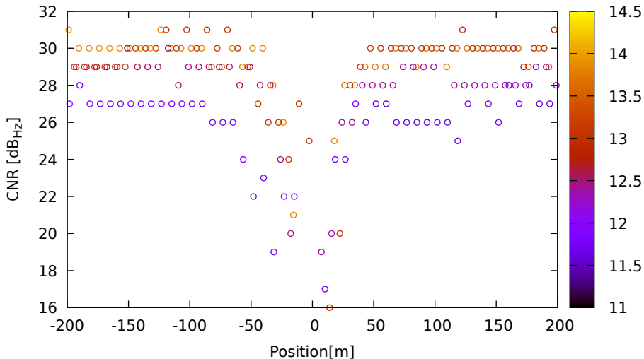
CNR vs position for G22 (L1) on HuaweiP40 - DOY 263 jam. 2
