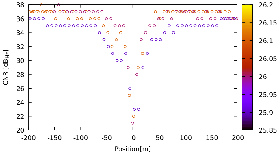
CNR vs position for G31 (L1) on HuaweiP40 - DOY 263 jam. 1
