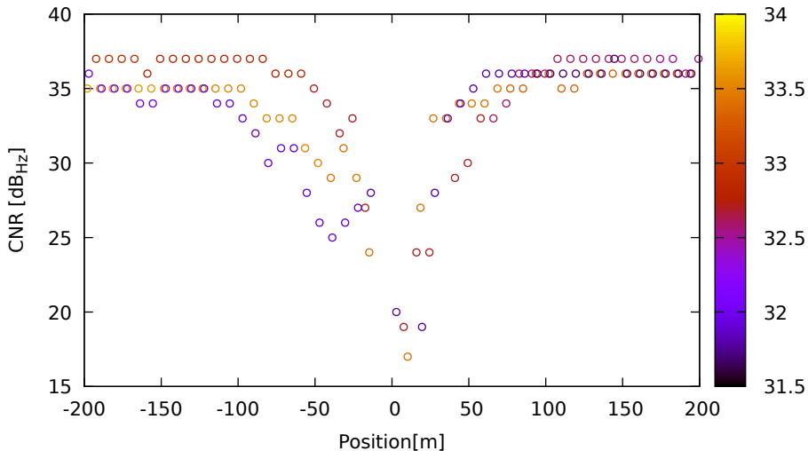
CNR vs position for R01 (G1) on HuaweiP40 - DOY 263 jam. 1
