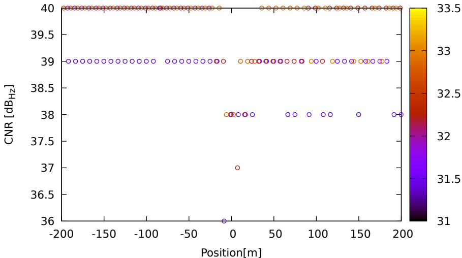
CNR vs position for R03 (G1) on HuaweiP40 - DOY 263 jam. 3
