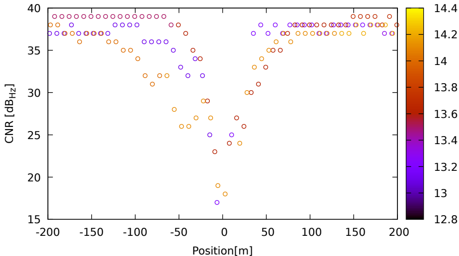
CNR vs position for R11 (G1) on HuaweiP40 - DOY 263 jam. 1
