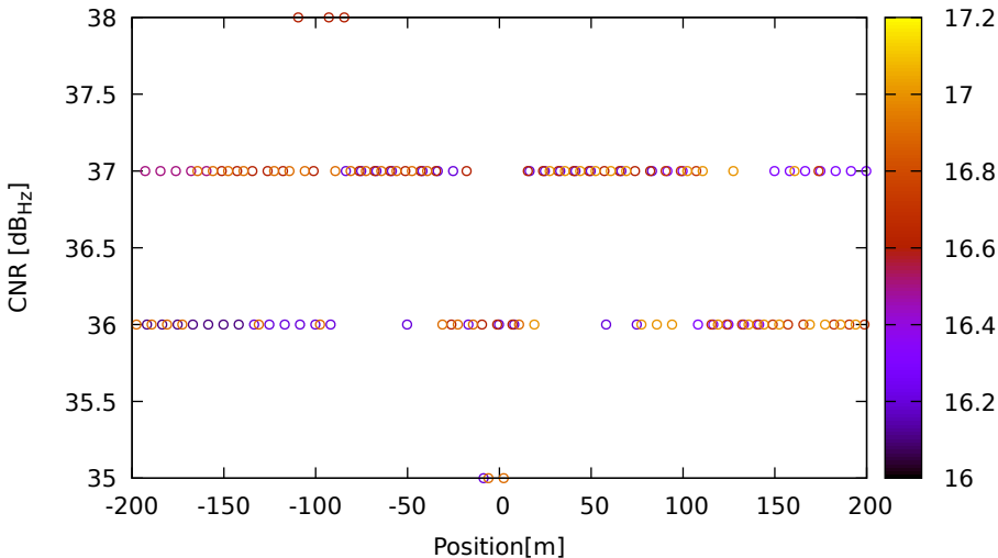
CNR vs position for R11 (G1) on HuaweiP40 - DOY 263 jam. 3
