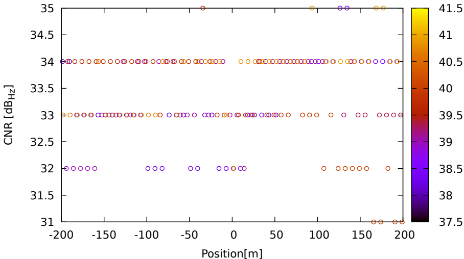
CNR vs position for R18 (G1) on HuaweiP40 - DOY 263 jam. 2
