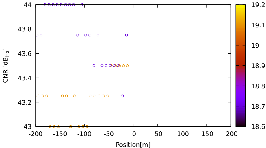
CNR vs position for C16 (B2) on LeicaGS18 - DOY 263 jam. 2
