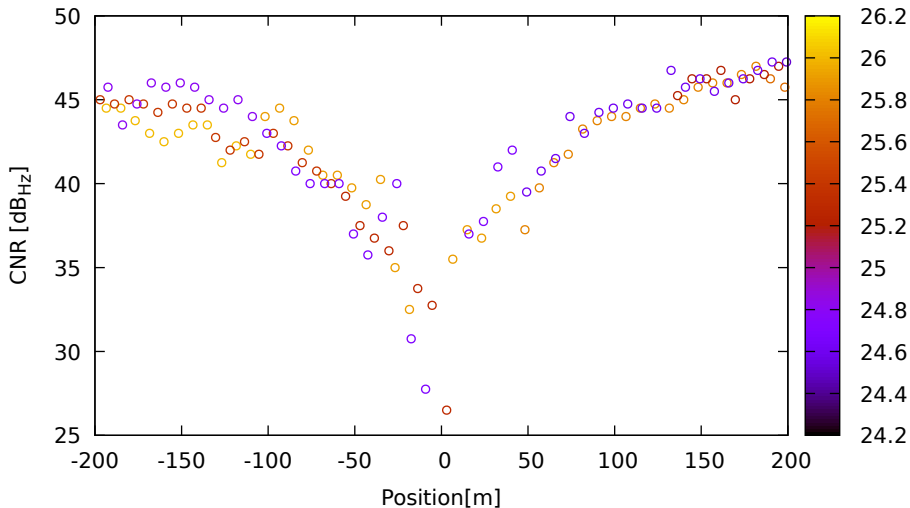
CNR vs position for C21 (B1) on LeicaGS18 - DOY 263 jam. 1
