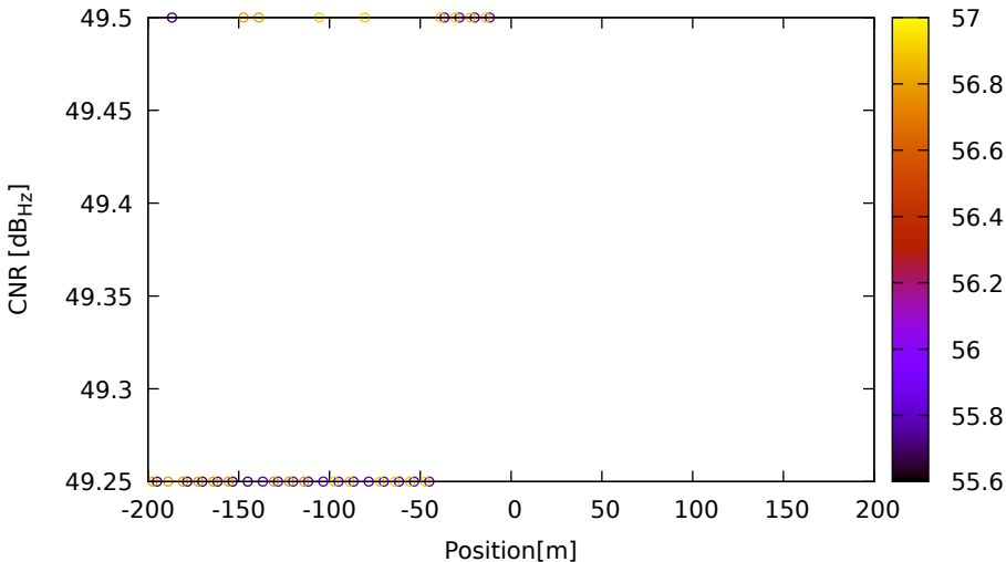
CNR vs position for E11 (E5b) on LeicaGS18 - DOY 263 jam. 2
