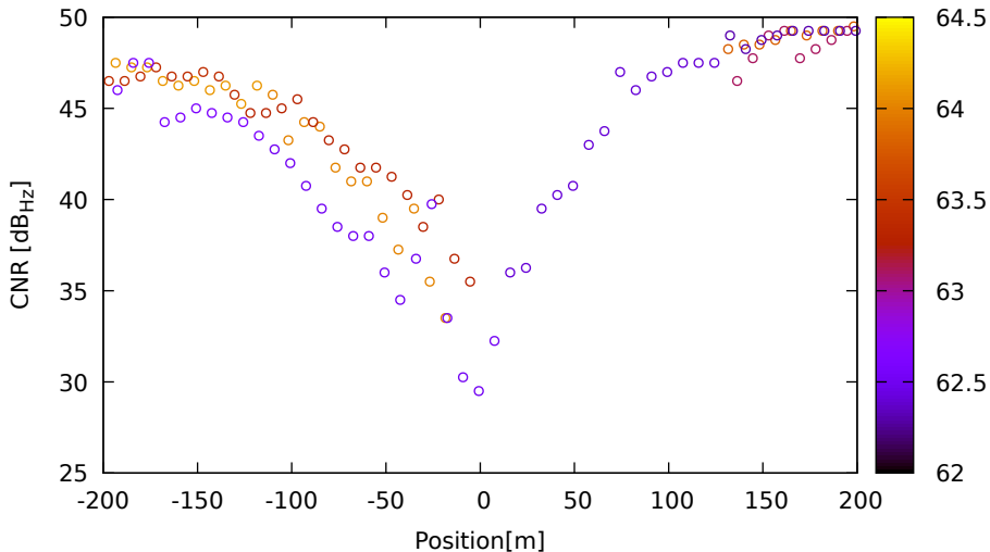
CNR vs position for E12 (E1) on LeicaGS18 - DOY 263 jam. 1
