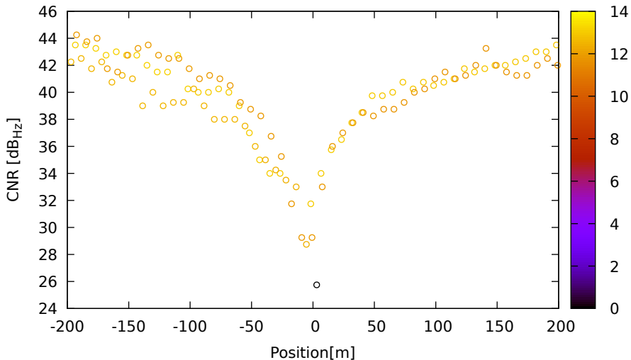
CNR vs position for E33 (E5b) on LeicaGS18 - DOY 263 jam. 1
