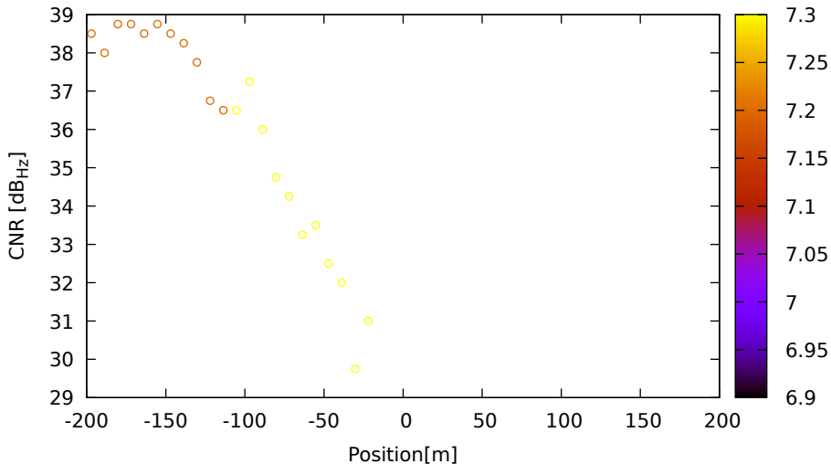
CNR vs position for E36 (E1) on LeicaGS18 - DOY 263 jam. 1
