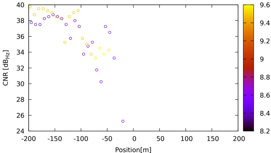
CNR vs position for E36 (E1) on LeicaGS18 - DOY 263 jam. 2
