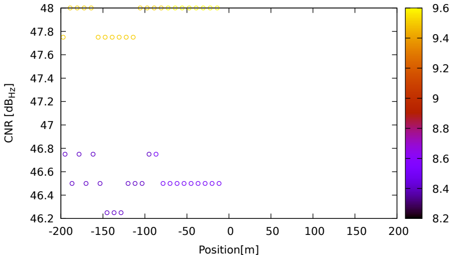
CNR vs position for E36 (E5) on LeicaGS18 - DOY 263 jam. 2
