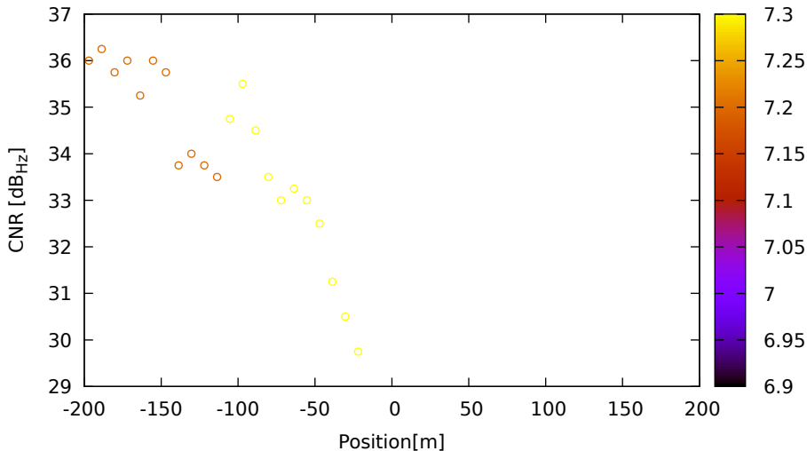
CNR vs position for E36 (E5a) on LeicaGS18 - DOY 263 jam. 1
