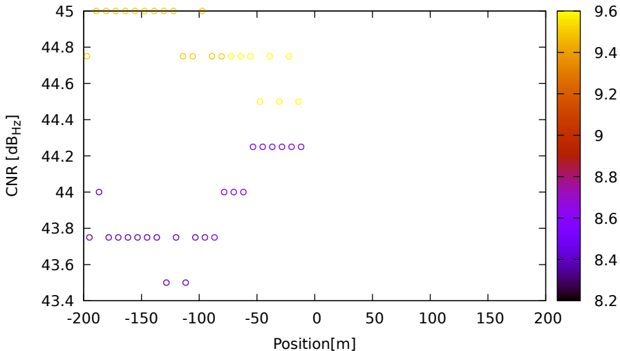
CNR vs position for E36 (E5b) on LeicaGS18 - DOY 263 jam. 2
