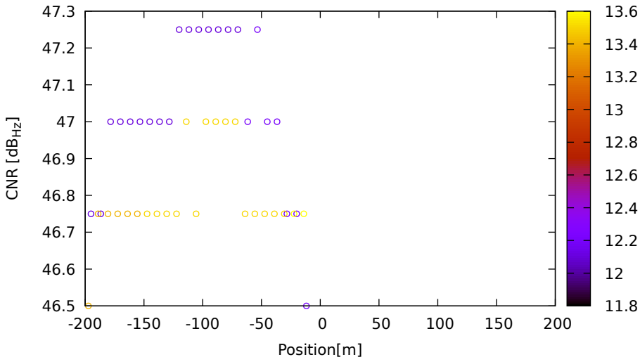
CNR vs position for G06 (L5) on LeicaGS18 - DOY 263 jam. 2
