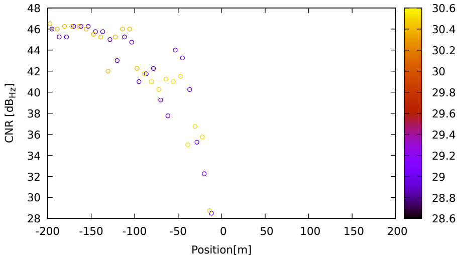
CNR vs position for G09 (L1) on LeicaGS18 - DOY 263 jam. 2
