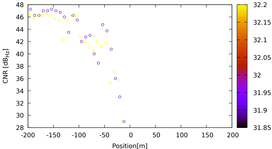
CNR vs position for G19 (L1) on LeicaGS18 - DOY 263 jam. 2
