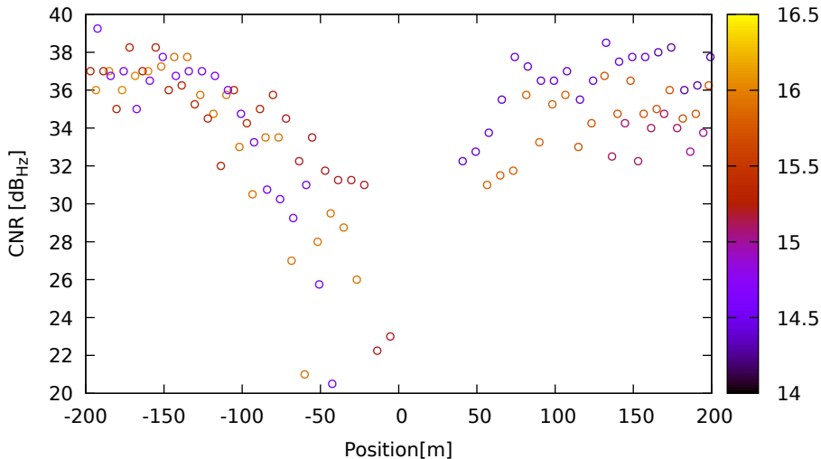
CNR vs position for G22 (L2) on LeicaGS18 - DOY 263 jam. 1
