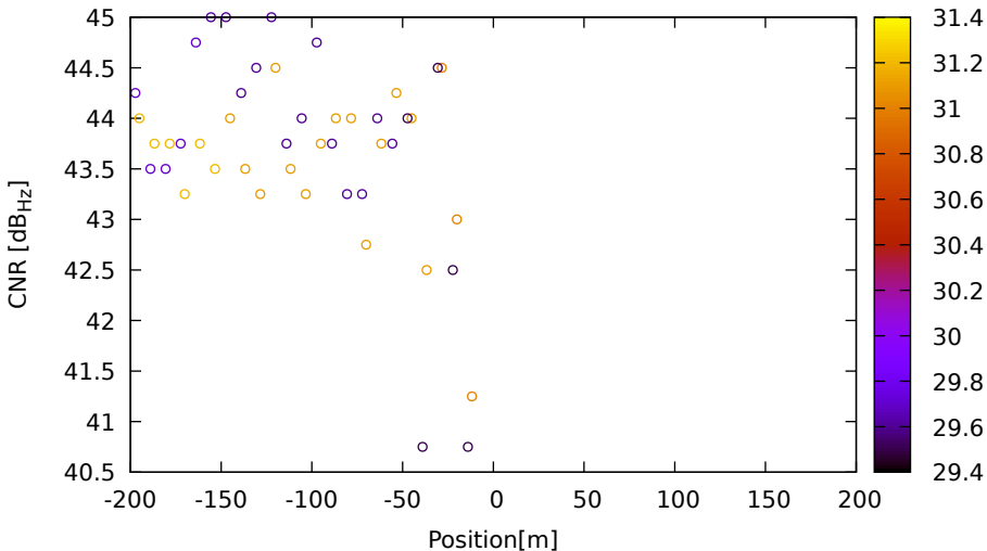
CNR vs position for R01 (G1) on LeicaGS18 - DOY 263 jam. 2
