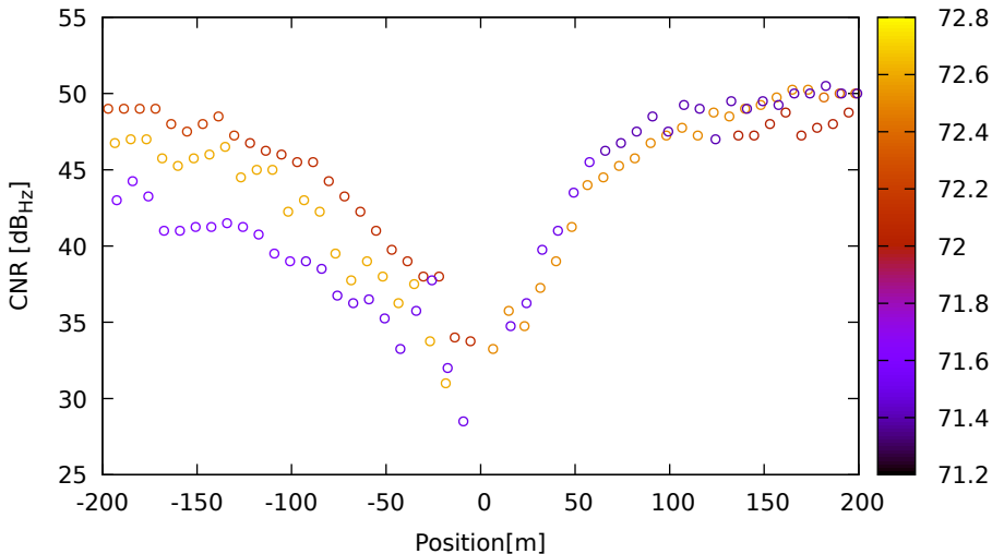
CNR vs position for R17 (G1) on LeicaGS18 - DOY 263 jam. 1
