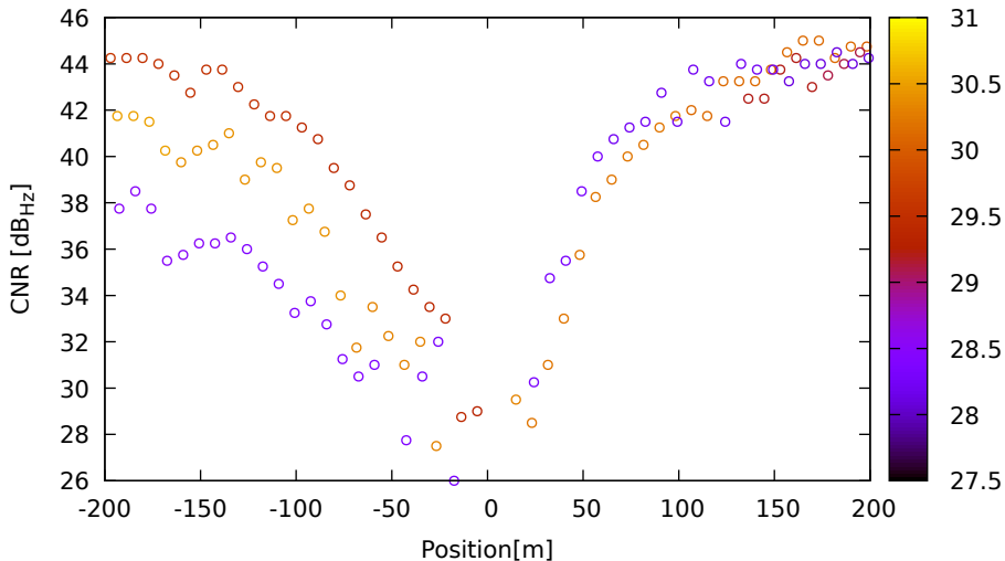
CNR vs position for R24 (G1) on LeicaGS18 - DOY 263 jam. 1
