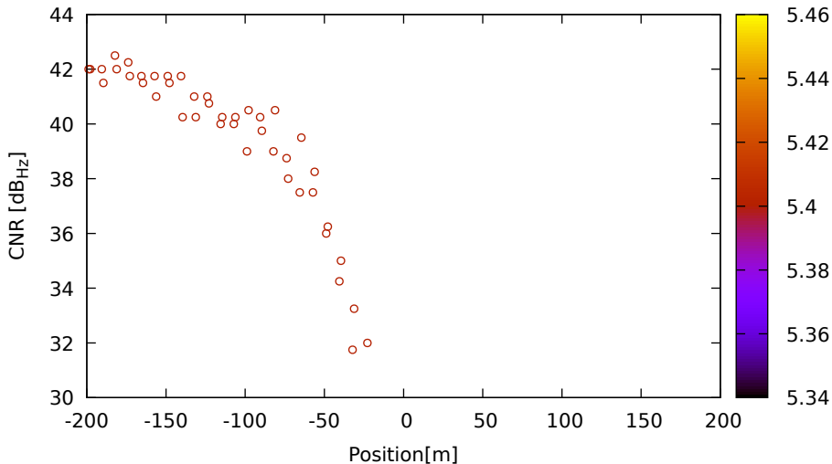
CNR vs position for C02 (B2) on LeicaGS18 - DOY 263 jam. 1
