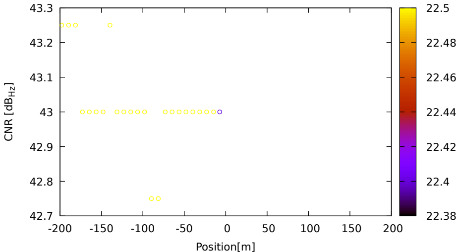
CNR vs position for C05 (B2) on LeicaGS18 - DOY 263 jam. 2
