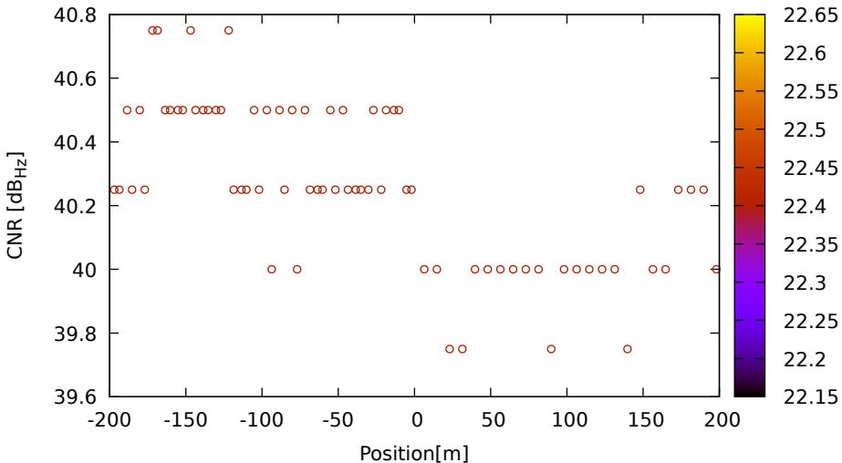
CNR vs position for C05 (B3) on LeicaGS18 - DOY 263 jam. 3
