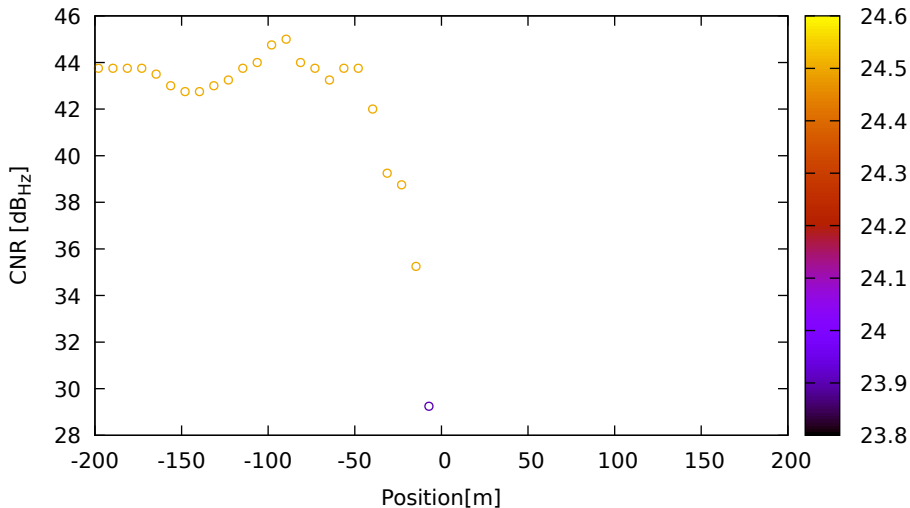
CNR vs position for C06 (B1) on LeicaGS18 - DOY 263 jam. 2
